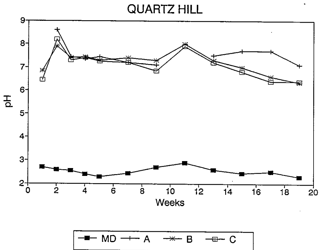
Figure 2. pH of mine drainage and permeameter effluents for National Tunnel and Quartz Hill Tunnel.
