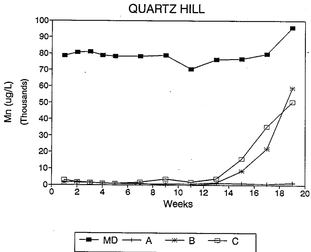
Figure 4. Manganese content of mine drainage and permeameter effluents for National Tunnel and Quartz Hill Tunnel.
